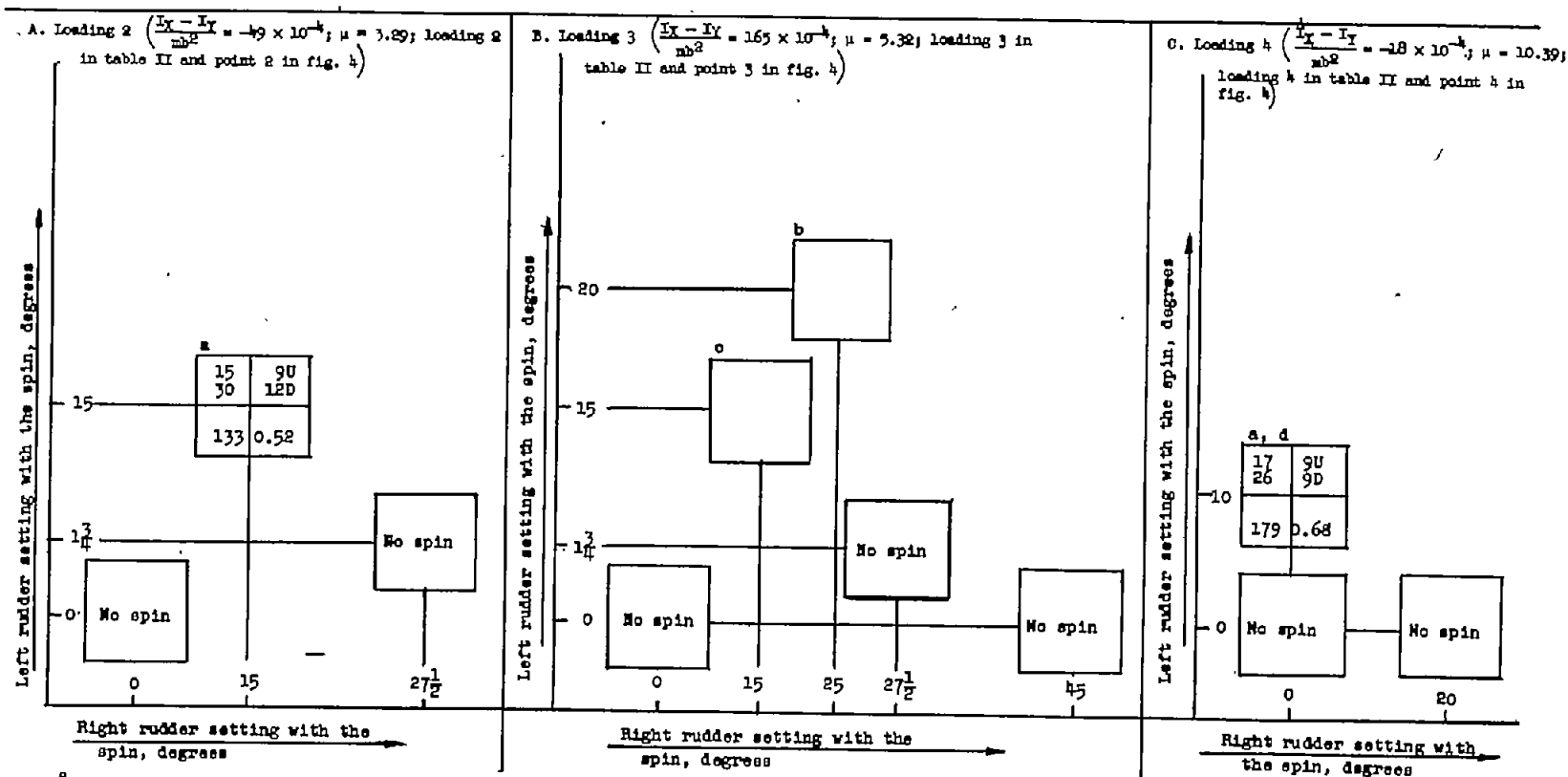
CHART 7.- EFFECT OF INDIVIDUAL AND COMBINED RUDDER DEFLECTIONS ON THE SPIN CHARACTERISTICS OF MODEL (RUDDERS AND AILERONS UNLATCHED)
