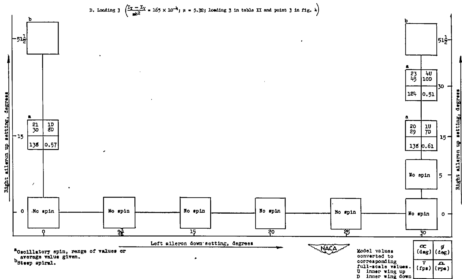
CHART 6.- EFFECT OF INDIVIDUAL AILERON DEFLECTIONS - Concluded
